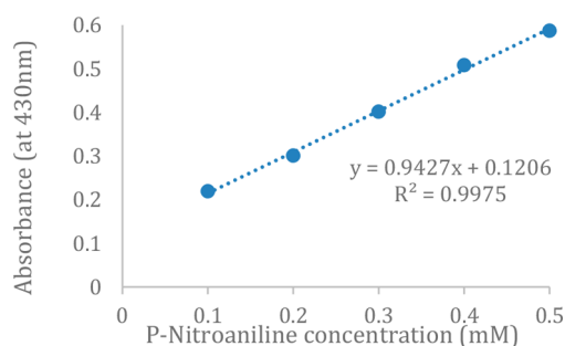
Figure 3. Calibration graph for p-nitroaniline for the shoebox spectrophotometer. Linear trend line equation and R^2 values are shown. Points are from a single observation, using water as a blank. Approximate wavelength determined as indicated in Validation section.
