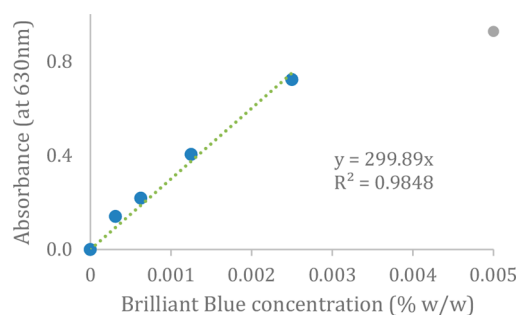
Figure 4. Calibration graph for Brilliant Blue for the shoebox spectrophotometer (blue ●). Linear trend line equations and R^2 values are shown. The gray ● represents a data point eliminated from the trend line equation due to a clear negative deviation. Points are from a single observation, using water as a blank. Approximate wavelength determined as indicated in Validation section.
