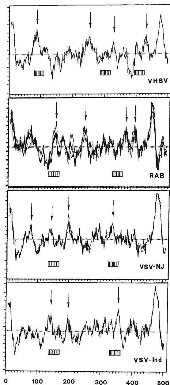
Fig. 3. Hydrophobic profiles and location of the heptad-repeats. The hydrophobic profiles from most of the sequences in Table 1 were obtained with the program SOAP from PCGene (Intelligenetics). The profiles from the different isolates or serotypes from VHSV, rabies, VSV-NJ, and VSV-Indiana were superimposed and the figures obtained are shown. The vertical arrows indicate the position of the highest hydrophobic peaks, whereas horizontal bars show the position of the heptad-repeats. The y axis shows the hydrophobic scales, and the X axis shows the amino-terminal position of the amino acids of rhabdovirus glycoprotein G.
