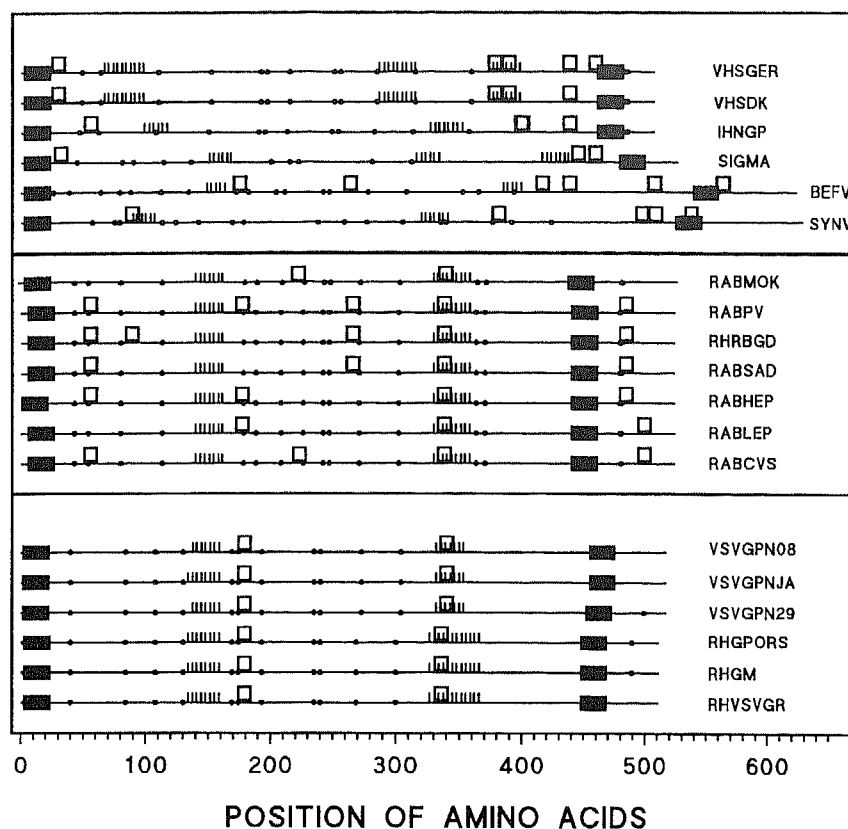
Fig. 1. Sequences of amino-terminal and carboxy-terminal a-d heptad-repeats in rhabdovirus glycoprotein G. The heptad-repeats (||||) were located by using the program PSEARCH (PCGene package, Intelligenetics). -\Delta G values \geq 0.4 kcal/mol for transfer of the amino acid side chain from water to ethanol were used to define the hydrophobic amino acids (single-letter code aa, W, F, Y, I, L, V, M, A, H, T) (14). The subsequence used for the search was (hydrophobic aa) XX (hydrophobic aa) XXX, repeated two times (X for any aa). Then the positions where more than 2 heptad-repeats were successively found in the glycoprotein G sequence were selected. The highly hydrophobic and continuous hydrophobic aa sequences of the predicted transmembrane and signal peptide regions were not considered. Symbols indicate cysteine (●), putative carbohydrate (□), and predicted transmembrane and signal peptide (■) relative positions in rhabdoviral glycoprotein G. The names of the rhabdoviruses are explained in Table 1.
