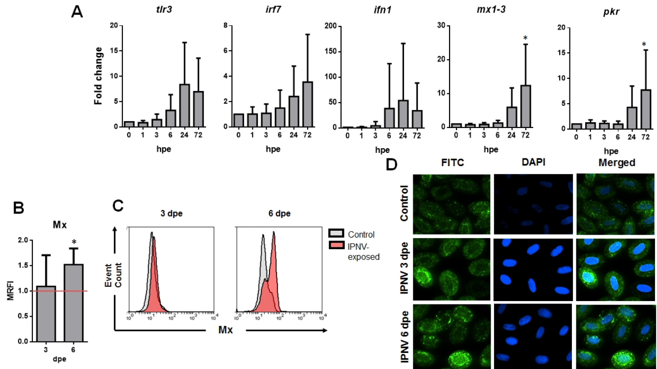
Figure 2. RBCs IFN-related antiviral response against IPNV. (A) Gene expression of tlr3 , irf7 , ifn1 , mx1-3 and pkr in IPNV-exposed RBCs at the indicated times post-infection and MOI 0.5, measured by RT-qPCR. Data represent mean \pm SD (n = 6). Kruskal-Wallis Test with Dunn's Multiple Comparison post-hoc test was performed among all time-points post-exposure in comparison with control time point (0 hpi) (*, p-value < 0.05). (B) Mx protein MRFI (mean relative fluorescent intensity, relative to control cells) in IPNV-exposed RBCs at MOI 0.5 (n = 5). (C) Flow cytometry histograms of Mx protein expression from control (grey) and IPNV-exposed (red) RBCs at MOI 0.5 and the indicated days post-exposure (dpe). (D) Representative immunofluorescence images of Mx protein expression in control and IPNV-exposed RBCs at MOI 0.5 (FITC – Mx protein expression, DAPI – Nuclei) (IF representative of 40 images).
